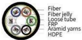
GCYF(X)Y Air-blown micro-cable
